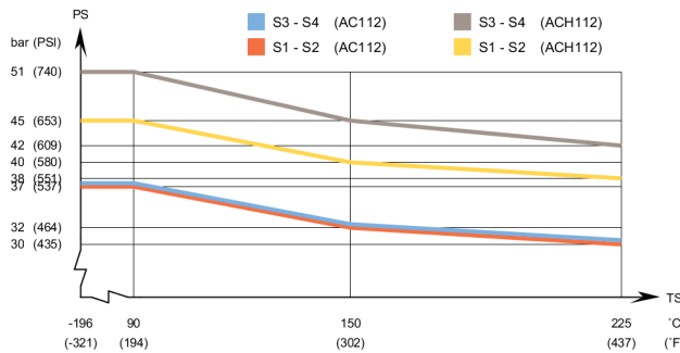
AC112 - PED approval pressure/temperature graph
